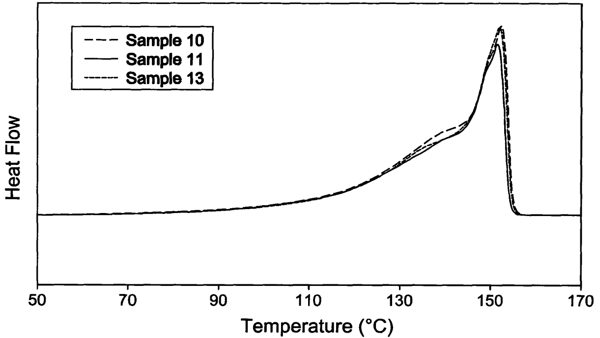
Fig. 7 DSC Melting of Plasticized Propylene Random Copolymers
